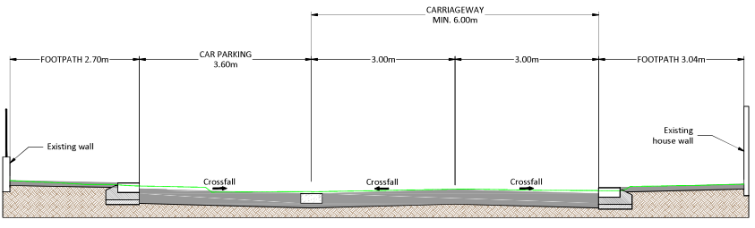
TYPICAL CROSS SECTION G-G SCALE 1:50
