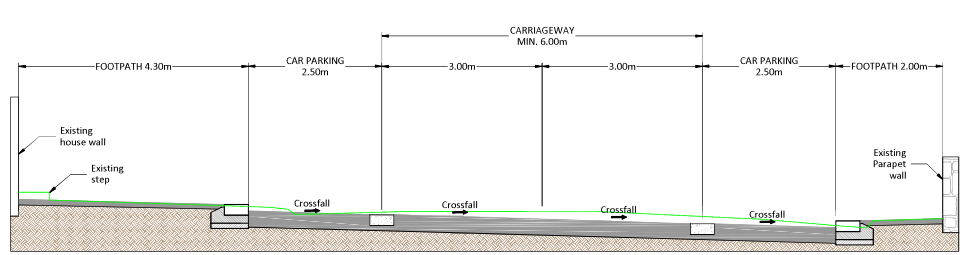
TYPICAL CROSS SECTION H-H SCALE 1:50
